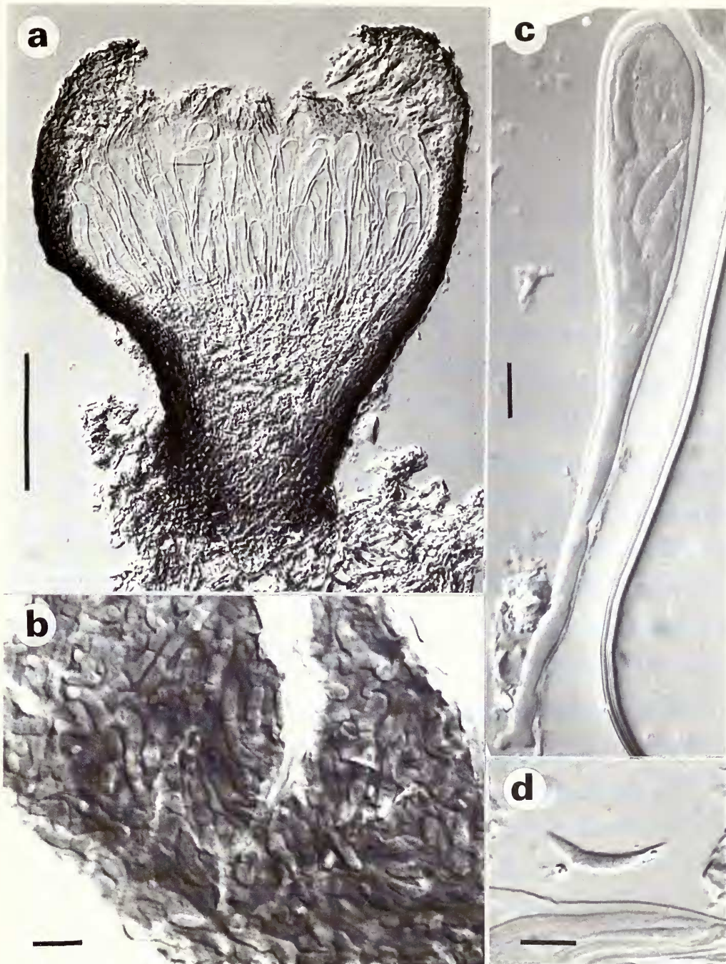
Fig. 65 Lahmia kunzei Körber (IMI 322591) (a) Vertical section of ascoma; scale = 100 \mu\text{m} ; (b) Detail of wall: textura intricata; (c) Ascus and ascospores; (d) Ascospore; scale = 10 \mu\text{m} .
